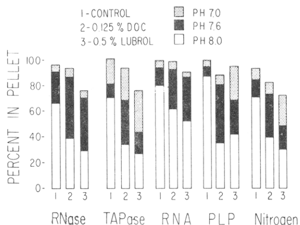
FIG. 3.—Solubilization of microsomal components by detergents. Washed beef pancreas microsomes were resuspended in mM phosphate, pH 7.0, and brought to 0.125% deoxycholate or 0.5% lubrol. The suspensions were then adjusted to pH 7.0, 7.6, or 8.0 and centrifuged at 90,000 \times g for 75 minutes. The pellets and supernatant solutions were each analyzed for total nitrogen, phospholipid phosphorus (PLP), RNA and RNase, and trypsin-activated protease (TAPase) activities.
